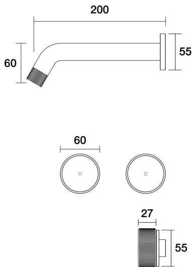
Opus Wall Basin Set 200mm Outlet B45.152.1.43 - Brass
