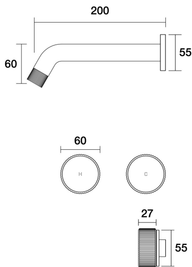
Opus Wall Basin Set 200mm Outlet Lane B45.152.2.45 - Native Brass
