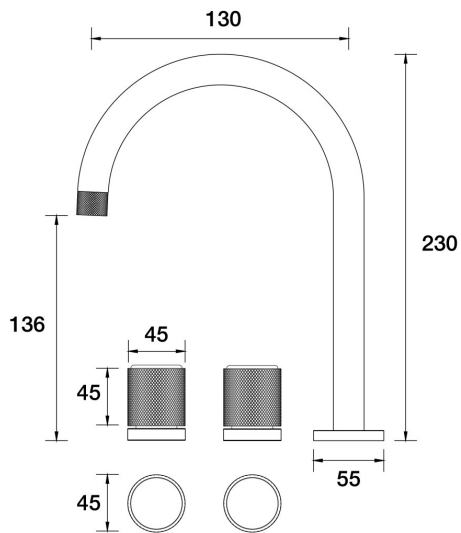
IDK Vetro Basin Set . B48.011.1.02 - Brushed Chrome
