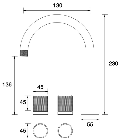
IDK Vetro Basin Set . B48.011.1.12 - 23k Brushed Gold
