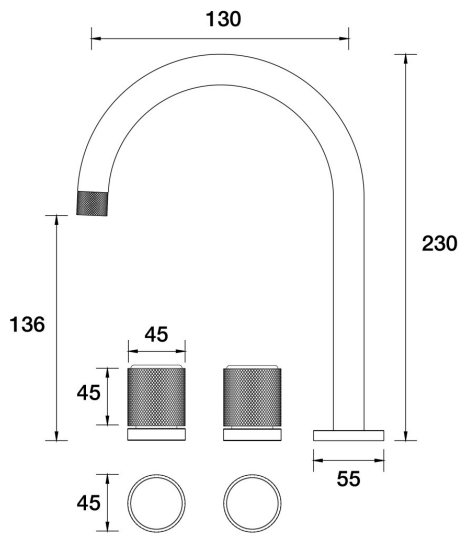
IDK Vetro Basin Set . B48.011.1.19 - 23k Brushed Brass Gold
