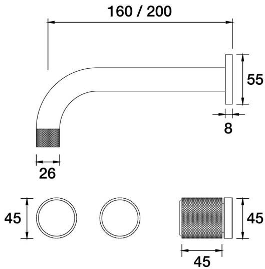
IDK Vetro Wall Bath Set . 160mm B48.021.1.01 - Chrome
