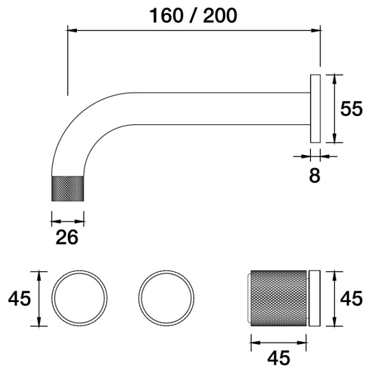
IDK Vetro Wall Bath Set . 200mm B48.021.2.45 - Native Brass
