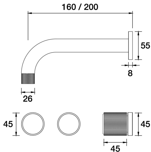
IDK Vetro Wall Bath Set . 200mm B48.021.2.67 - Vintage Brass
