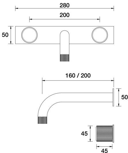
IDK Vetro Wall Bath Set . on plate 200mm B48.021.4.01 - Chrome
