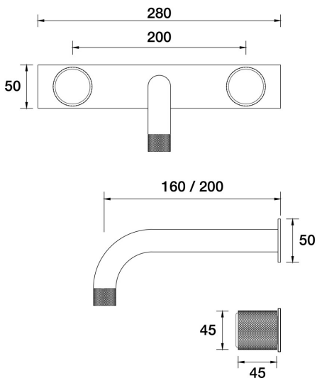
IDK Vetro Wall Bath Set . on plate 200mm B48.021.4.41 - Brushed Brass
