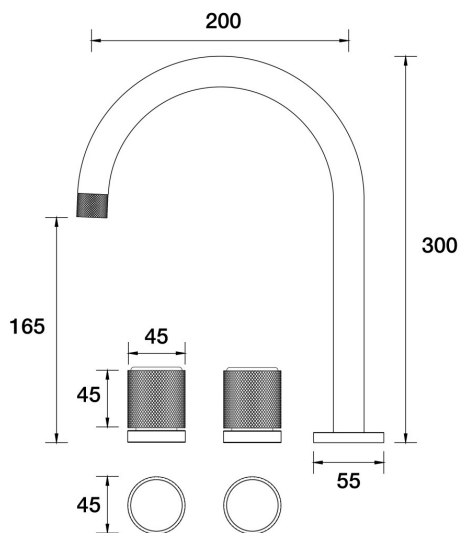
IDK Vetro Spa Set Hob B48.061.1.11 - 23k Gold
