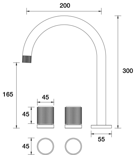
IDK Vetro Spa Set Hob B48.061.1.67 - Vintage Brass
