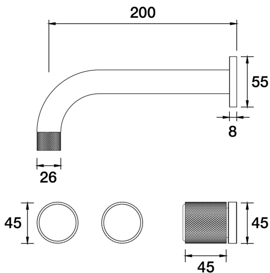
IDK Vetro Wall Basin Set . B48.152.1.01 - Chrome
