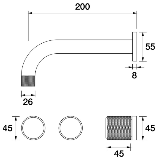
IDK Vetro Wall Basin Set . B48.152.1.48 - Copper
