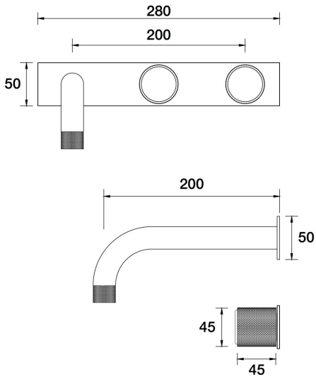
IDK Vetro Wall Basin Set . On Plate Offset B48.152.3.39 - Antique Bronze
