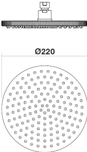
Universal Shower Rose Round 220mm IDK C11.081.2.01 - Chrome
