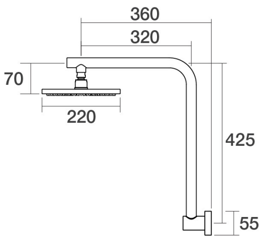
Lugano Fixed Wall Arm Shower Hi Rise Shower 90° C22.011.2.01 - Chrome
