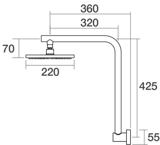
Lugano Fixed Wall Arm Shower Hi Rise Shower 90° C22.011.2.45 - Native Brass
