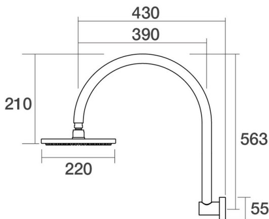
Lugano Fixed Wall Arm Shower Hi Rise Gooseneck C22.011.3.47 - Luminick
