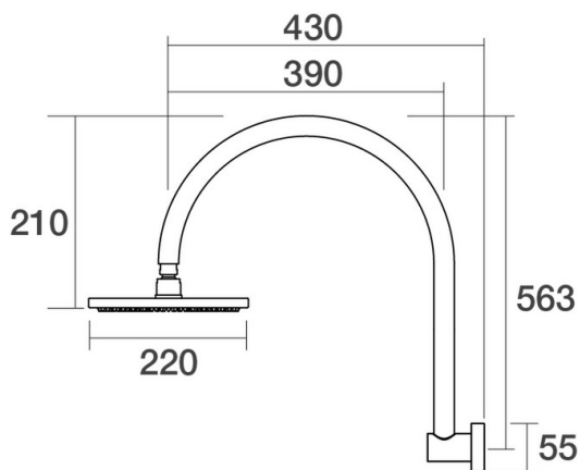
Lugano Fixed Wall Arm Shower Hi Rise Gooseneck C22.011.3.68 - Autumn Bronze
