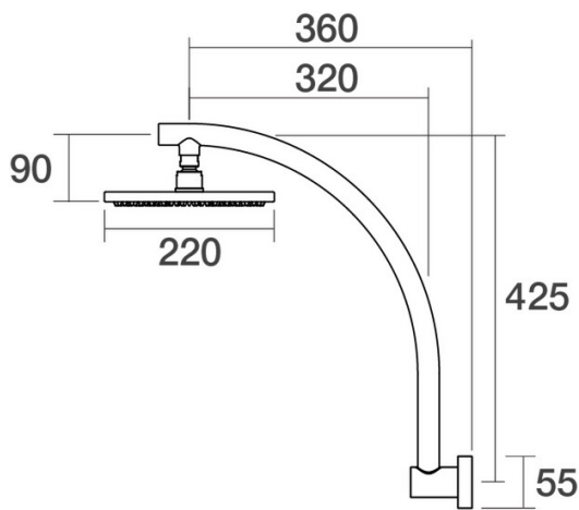
Lugano Fixed Wall Arm Shower Hi Rise Arc C22.011.4.25 - Brushed Nickel
