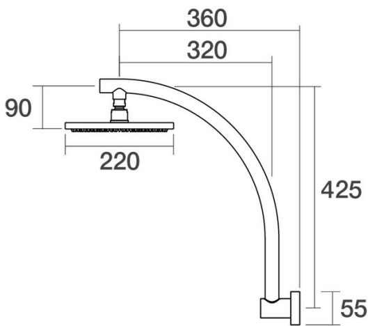
Lugano Fixed Wall Arm Shower Hi Rise Arc C22.011.4.70 - Sea Spray
