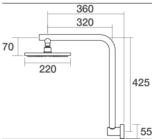
Lugano Wall Fixed Arm with 220mm Rose Hi Rise 90° C22.011.5.01 - Chrome
