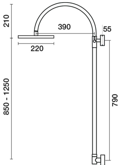
Lugano Wall Exposed Shower with 220mm Rose Adjustable Height C22.031.1.01 - Chrome
