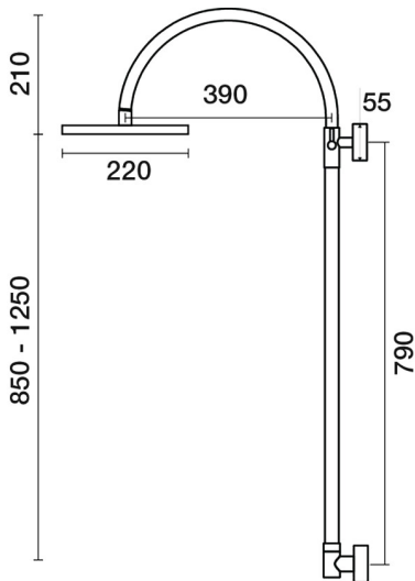
Lugano Exposed Wall Shower Adjustable Height C22.031.1.57 - Matt Nickel
