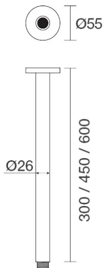
Lugano Ceiling Drop Arm 450mm C22.041.3.23 - Gunmetal
