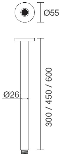
Lugano Ceiling Drop Arm 600mm C22.041.4.26 - Black Sapphire
