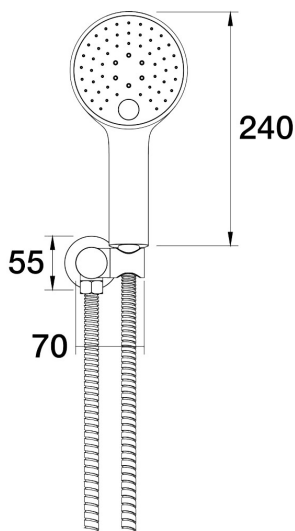
Lugano Handshower on Wall Bracket Three Function 0220011.24 - Brushed Gunmetal
