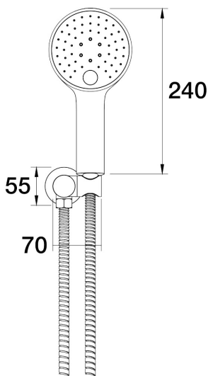
Lugano Handshower on Wall Bracket Three Function 0220011.40 - Rumbled Brass
