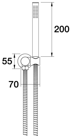
Lugano Handshower on Wall Bracket Single Function
