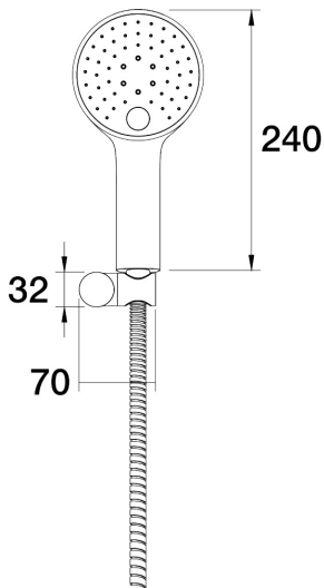
Lugano Handshower on Wall Bracket Three function without water connection C22.051.3.12 - 23k Brushed Gold
