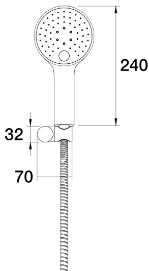
Lugano Handshower on Wall Bracket Three function without water connection C22.051.3.23 - Gunmetal
