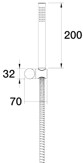
Lugano Handshower on Wall Bracket Single function without water connection C22.051.4.01 - Chrome
