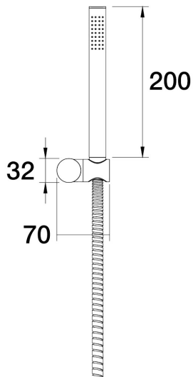
Lugano Handshower on Wall Bracket Single function without water connection C22.051.4.19 - 23k Brushed Brass Gold
