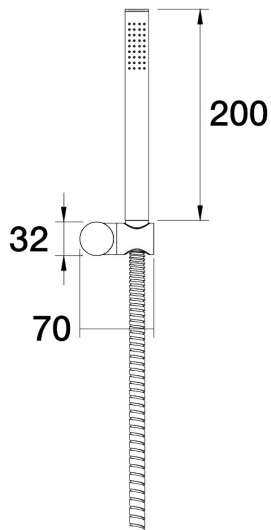
Lugano Handshower on Wall Bracket Single function without water connection C22.051.4.39 - Antique Bronze
