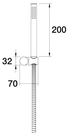
Lugano Handshower on Wall Bracket Single function without water connection C22.051.4.40 - Rumbled Brass
