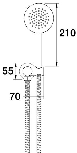
Lugano Handshower on Wall Bracket Handshower on Wall Bracket C22.051.5.45 - Native Brass
