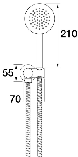
Lugano Handshower on Wall Bracket Handshower on Wall Bracket C22.051.5.67 - Vintage Brass
