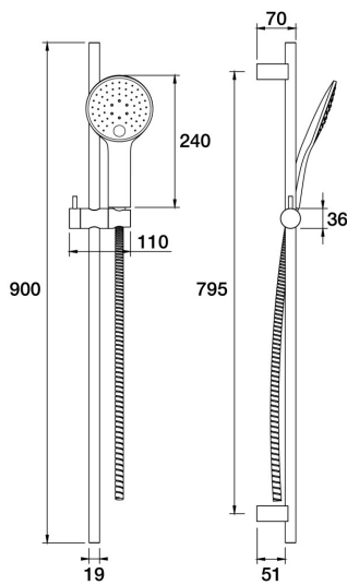
Lugano Handshower on Rail Three Function C22.052.1.19 - 23k Brushed Brass Gold
