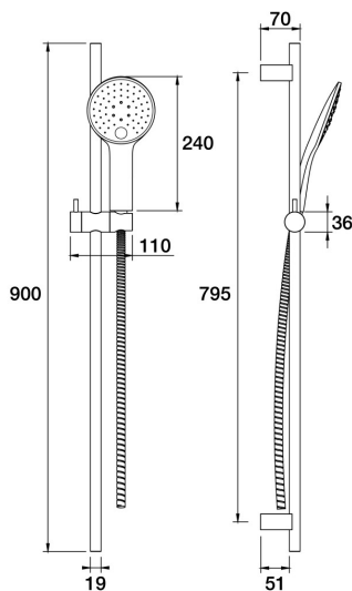
Lugano Handshower on Rail Three Function C22.052.1.26 - Black Sapphire
