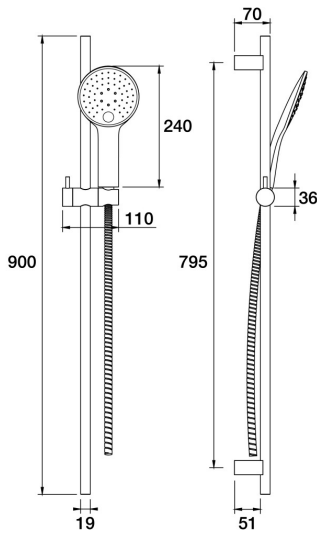
Lugano Handshower on Rail Three Function C22.052.1.43 - Brass
