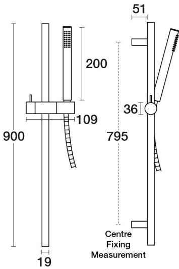
Lugano Handshower on Rail Single Function C22.052.2.01 - Chrome
