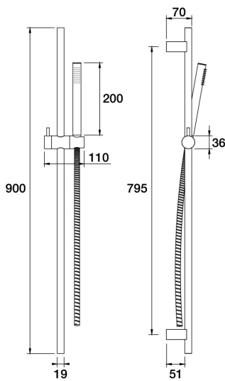
Lugano Handshower on Rail Single Function C22.052.2.12 - 23k Brushed Gold
