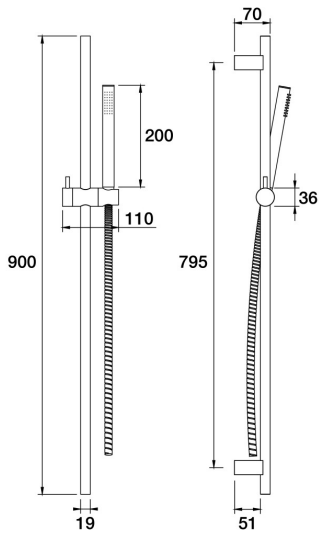
Lugano Handshower on Rail Single Function C22.052.2.42 - Brushed Copper
