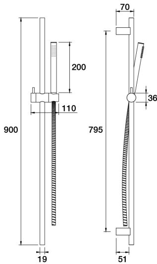
Lugano Handshower on Rail Single Function C22.052.2.67 - Vintage Brass
