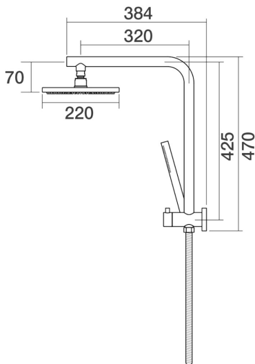
Lugano Wall Shower Divertor High Rise 90 Degree C22.061.1.11 - 23k Gold
