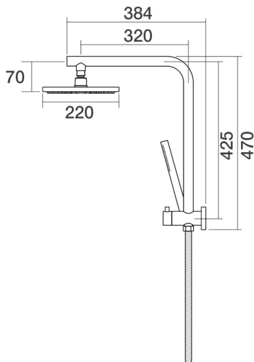
Lugano Wall Shower Diverter High Rise 90 Degree C22.061.1.19 - 23k Brushed Brass Gold
