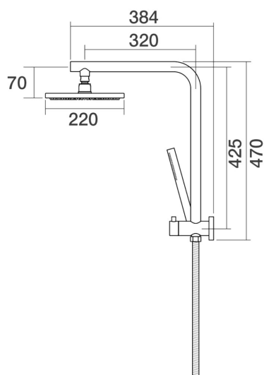
Lugano Wall Shower Divertor High Rise 90 Degree C22.061.1.27 - Satin Pearl
