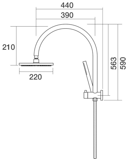
Lugano Wall Shower Diverter High Rise Gooseneck C22.061.2.44 - Antique Copper
