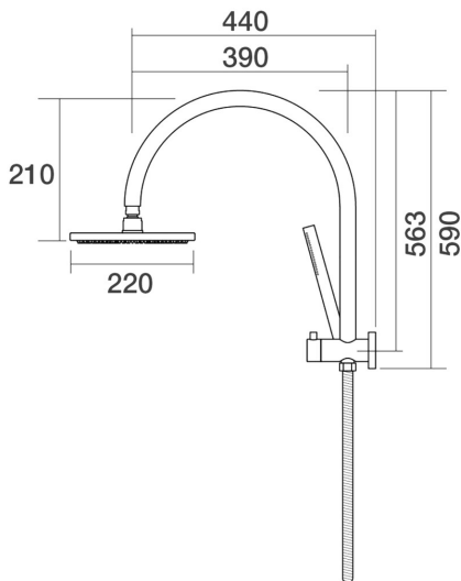
Lugano Wall Shower Divertor High Rise Gooseneck C22.061.2.54 - Volcanic Grey
